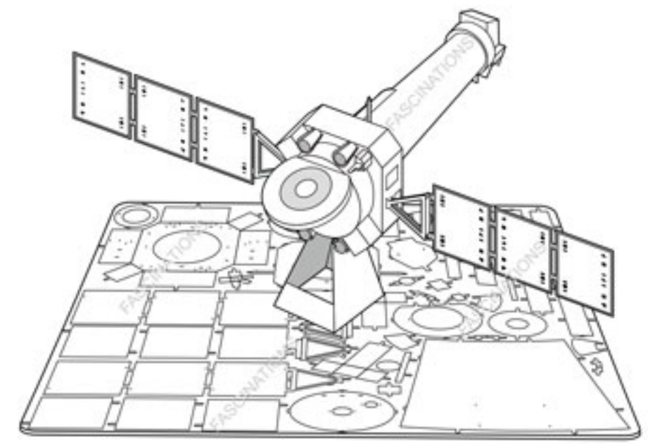
Chandra X-ray Observatory Item No. MMS174
